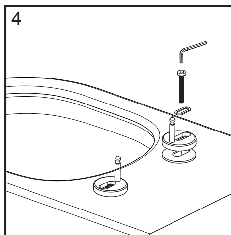
Fit the rubber pads to the underside of the 2 hinge mounting posts, insert the elongated washer and loosely fasten to the pan.
